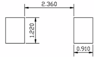
UNIT: mm SUGGESTED SOLDER PAD LAYOUT
