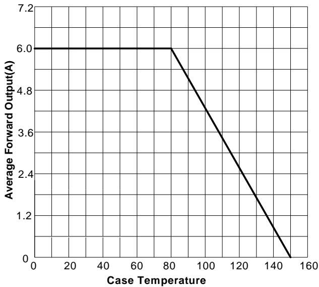
FIG1:Io-Tc Curve
