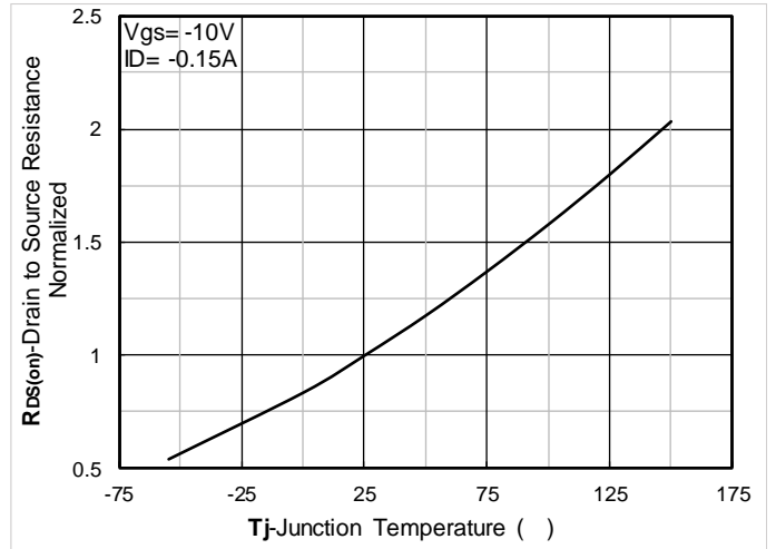
Figure8. Normalized On-Resistance
