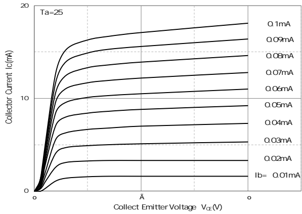
Static Characteristic
